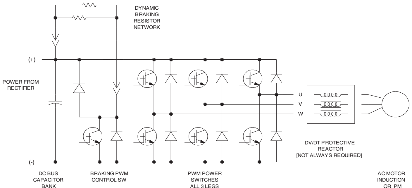
Figure 3 - Typical inverter power section
