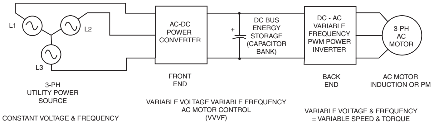
Figure 2 - Basic inverter control
